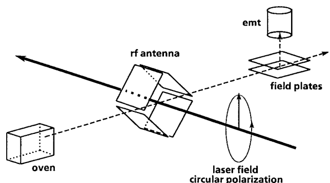
FIG. 3. Scheme of the experimental setup.
